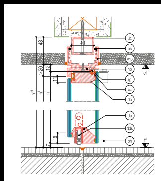
GM MARTITION® Light Drehtür
